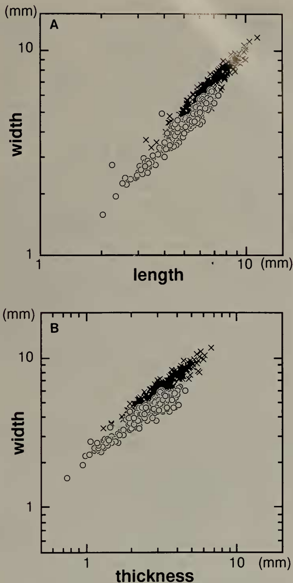
Figure 5. Scatter diagrams of A: length to width, and B: thickness to width, in Shimodaia pterygiota (×) (n=259), and Frenulina sanguinolenta (○) (n=230). Specimens of F. sanguinolenta used in this study were collected from "Tori-ike" cave, off Shimoji Islet, Miyako Island, Okinawa, at between 12 m and 40 m depth.
